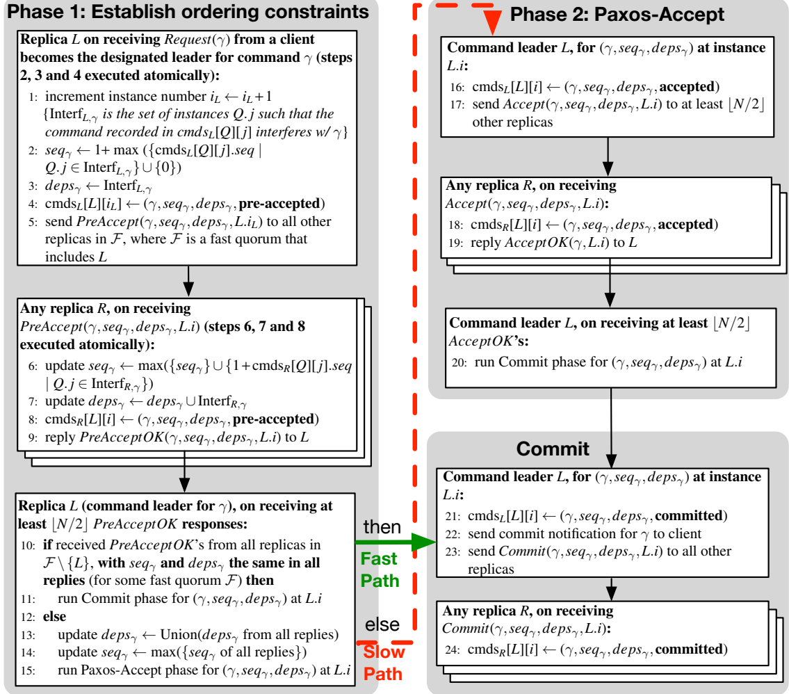
Figure 3.2: The basic Egalitarian Paxos protocol for choosing commands.
