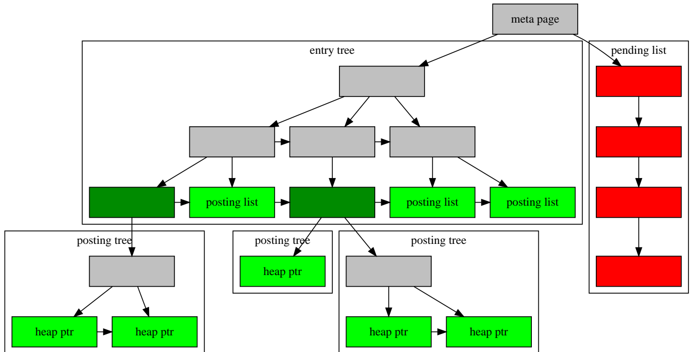
Figure 64.1. GIN Internals
