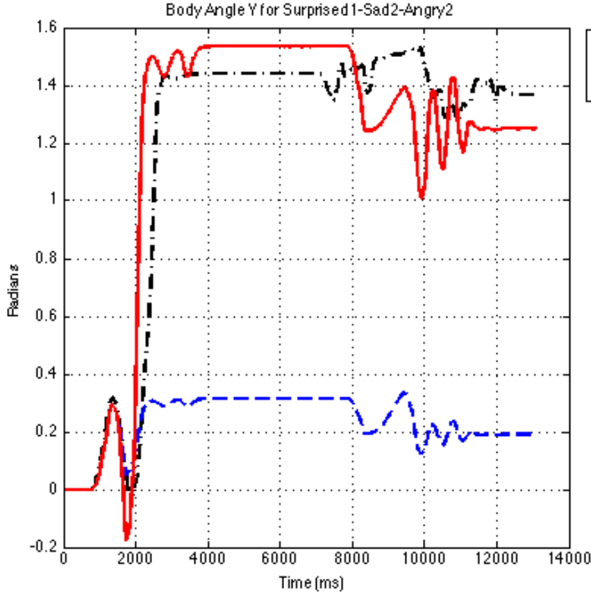
Figure 6.3: Body angle Y values for Sad2-Angry2-Surprised1 [Tay et al., 2016].
