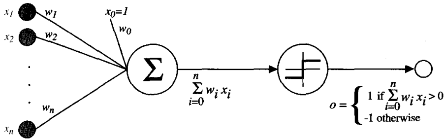
FIGURE 4.2 A perceptron.
