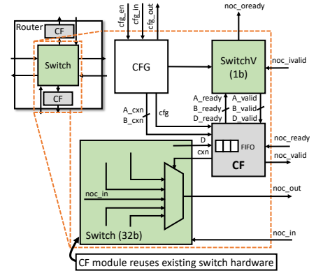
Figure 8: Router microarchitecture
