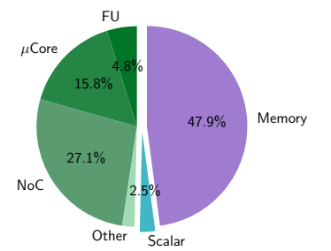
Figure 12: Area breakdown for a complete RipTide system. Area is dominated by the CGRA fabric and main memory (SRAM + arbitration logic), each taking about half of the system. The scalar core is just 2.5% of system area. The NoC takes 54% of CGRA area, and PEs ( \mu core + FUs) take 42%.
